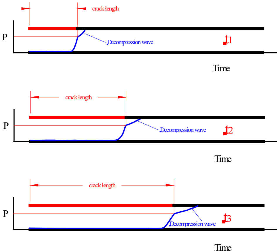
Figure G.3 A schematic of the pressure profile of a decompression wave travelling down a pipeline
