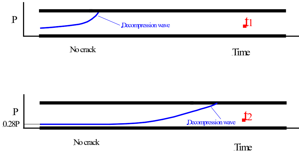
Figure G.2 A schematic of the pressure profile of a decompression wave travelling down a pipeline. For an infinitely long pipeline the pressure never reduces below 28% of the initial pressure for test gases nitrogen or air.
